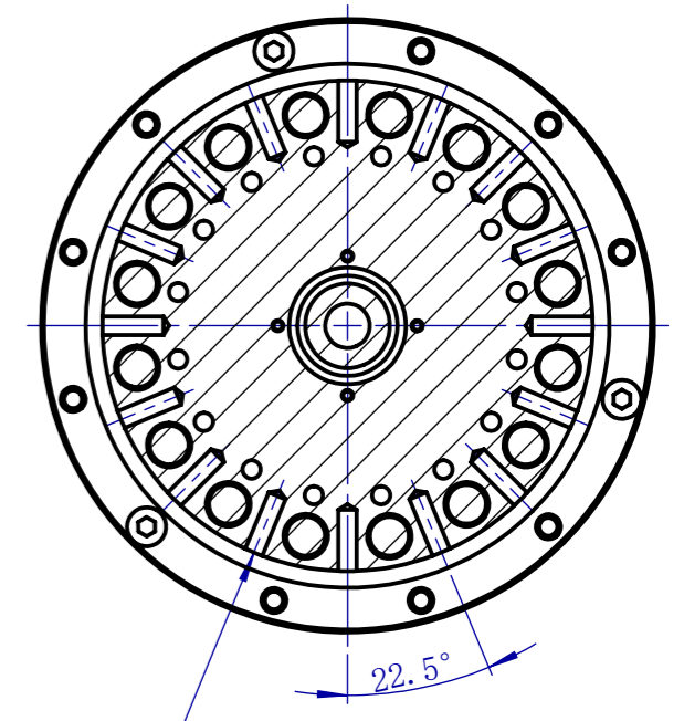
16 x M4 - 6H 均布 evenly distributed 输出法兰径向安装螺钉孔 Output flange radial mounting screw hole 剖面 A-A Section A-A 比例 1 : 1.5 Scale 1:1.5
